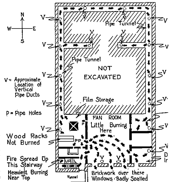
PLAN OF BASEMENT SHOWING HORIZONTAL SPREAD OF FUMES AND FIRE
