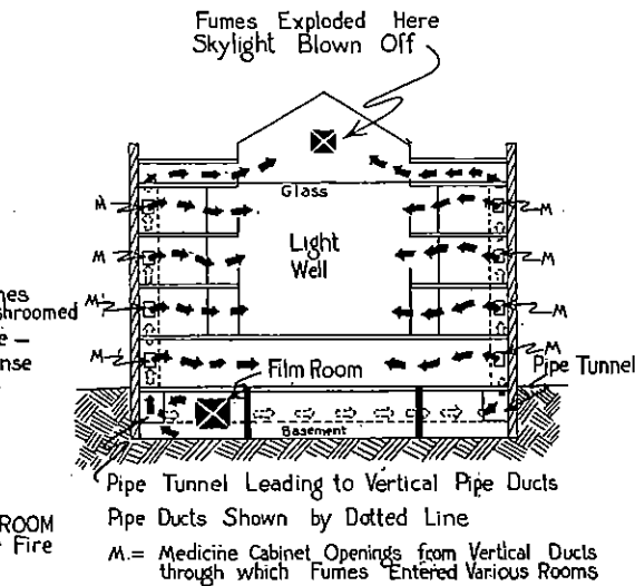
SECTION SHOWING HOW FUMES SPREAD VERTICALLY THROUGH BUILDING.
